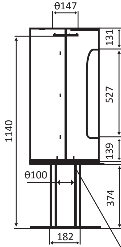
Central AIR INTAKE \theta 100 mm
