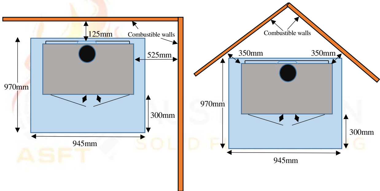
Figure 1 – Clearance Diagram
